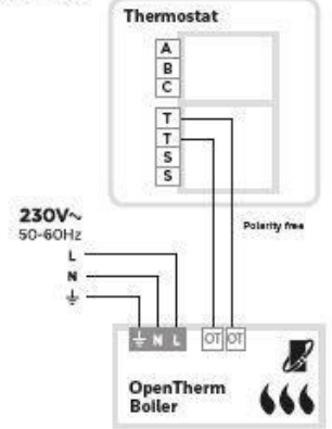
OpenTherm Boiler
