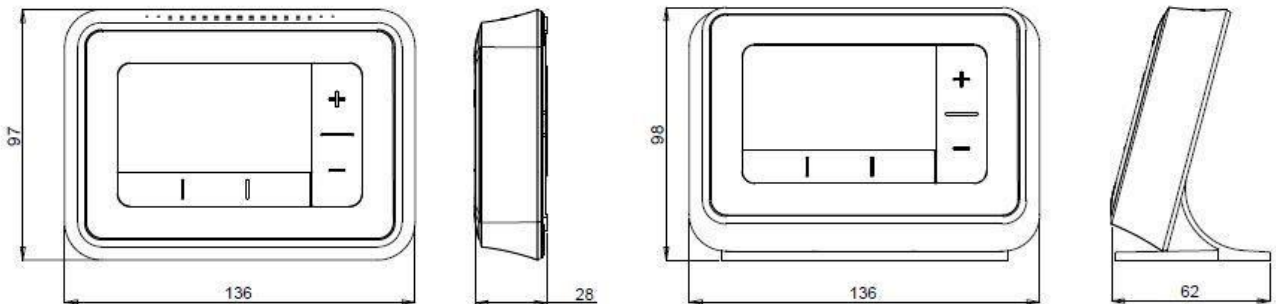
T4R THERMOSTAT
