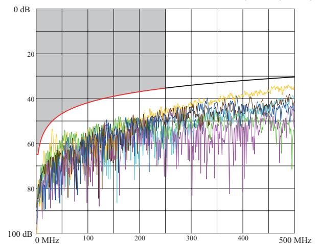
NEXT (Near end Crosstalk Attenuation) (Atténuation paradiaphonique)
