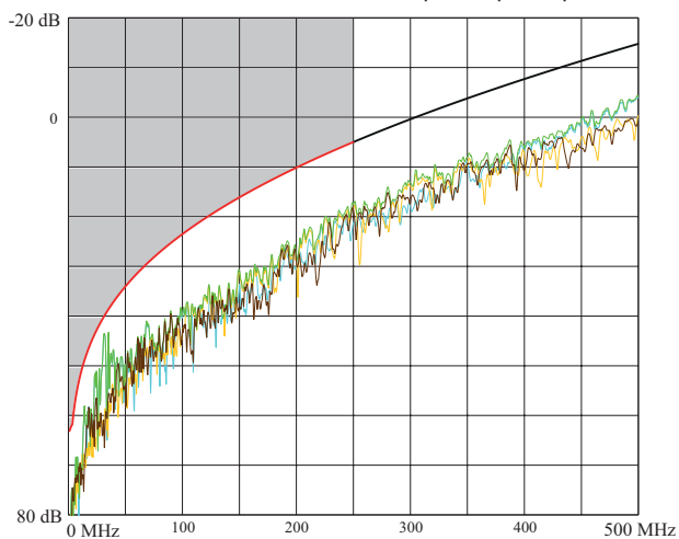
ACR (Attenuation to Crosstalk Ratio) (Ecart paradiaphonique)
