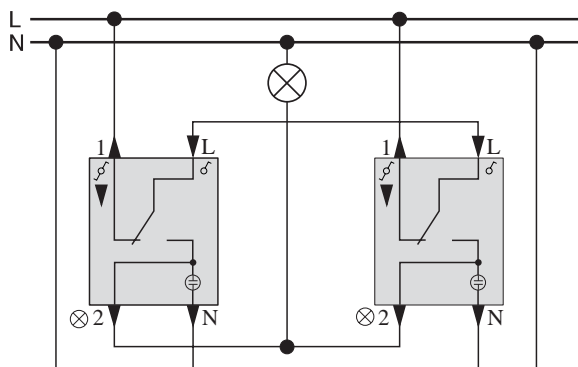
Two-way switch with indicator light Mxx3x06-0000
