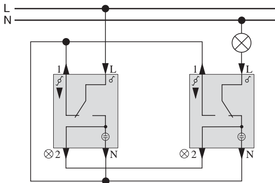
Two-way switch with indicator light Mxx3x06-0000
