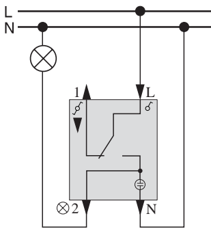
Two-way switch with indicator light Mxx3x06-0000
