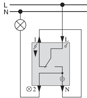
Two-way switch with indicator light Mxx3x06-0000
